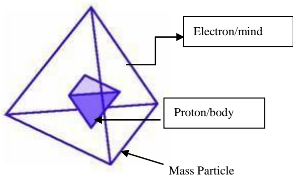
Figure 6. Mass particle is formed due to disorder in dark energy where dark energy content within two energy particles connected face to face combine with each other in one space under high compressive force from neighbouring energy particles. The union of two energy particles connected face to face lead to formation of a denser and lighter zone. The denser portion is proton that makes our body and the ray emitted from surface of portion, i.e. flow of electron that makes our mind. Within dense portion of dark energy summation of rays oscillates between two third and one third distance, i.e. from vertex to centroid and centroid to base due to confinement of two energy particles in one unit particle space. When two energy particles combine in nucleus one mass particle-hydrogen atom is formed but when two mass particle, i.e. two hydrogen atoms combine in nucleus, joining surface of two hydrogen atom become neutral due to interference of emitted rays of two surfaces and a new element is formed with two proton, two electron and two neutron. When two mass particle combine in earth one hydrogen molecule is formed. As one icosahedron shaped energy space have twenty energy particles so ten mass particle can be formed within that space with 2, 2, 6 electronic configuration
